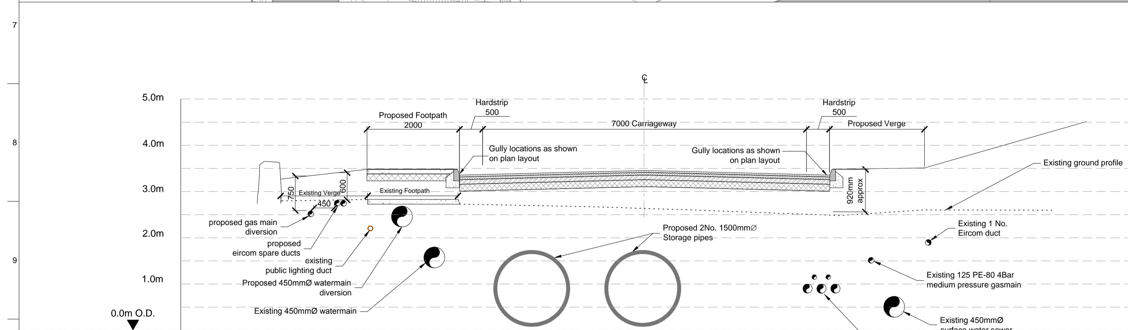
Proposed Road & Services - Section B-B Scale: 1:50
