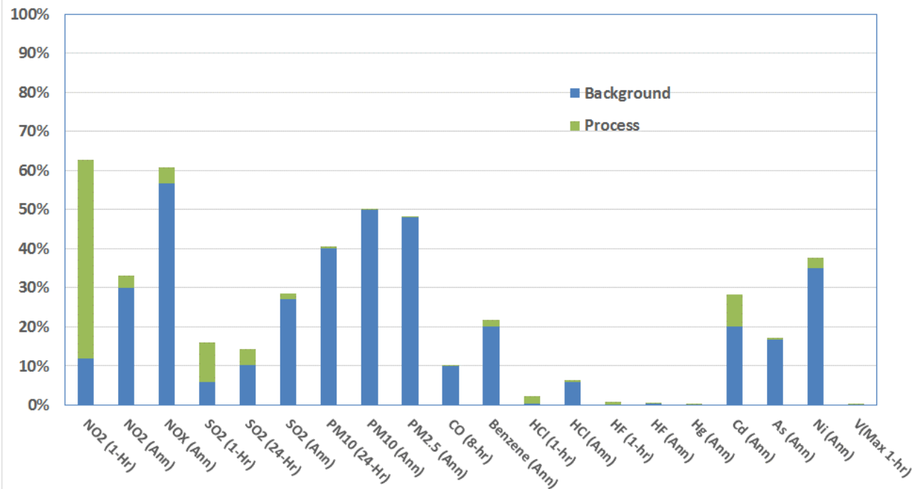
AERMOD Air Modelling Concentrations As A Percentage Of The Ambient Air Quality Standards
