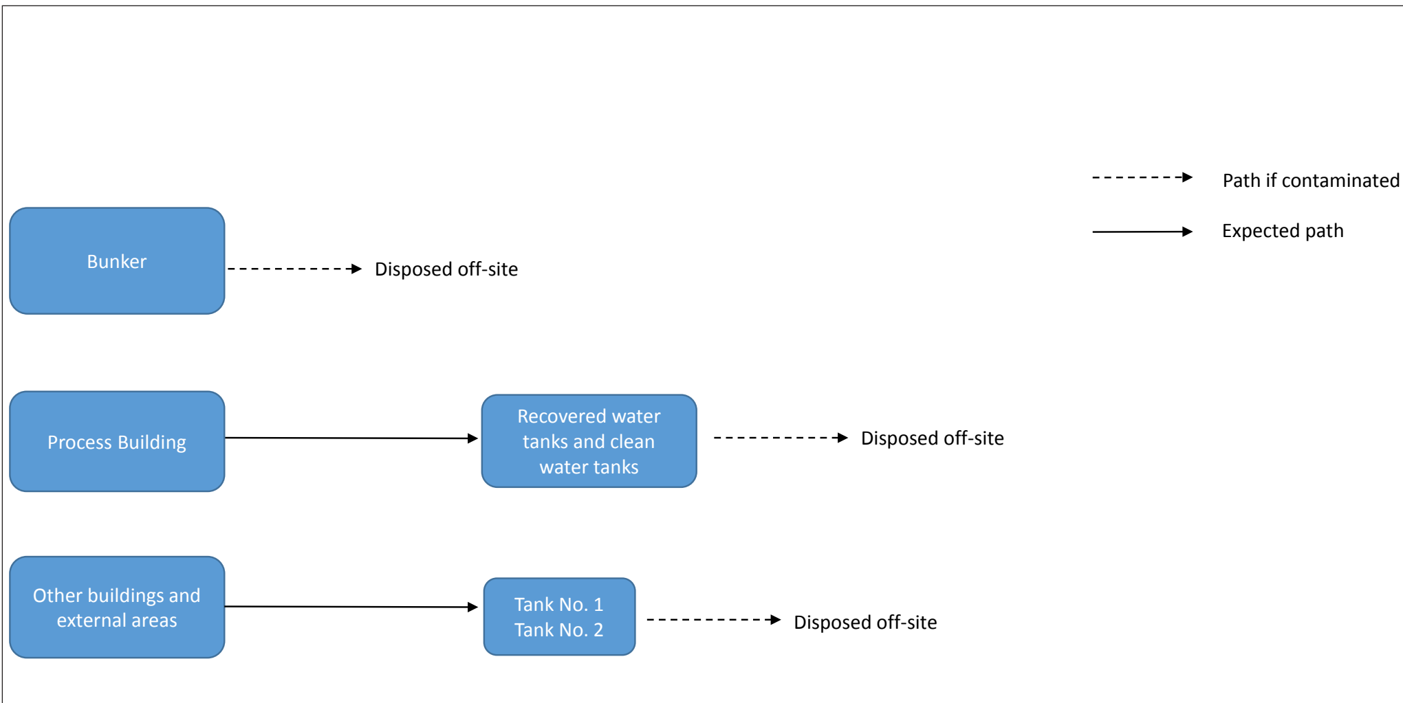
Figure 4.19 Schematic of Firewater Management System
