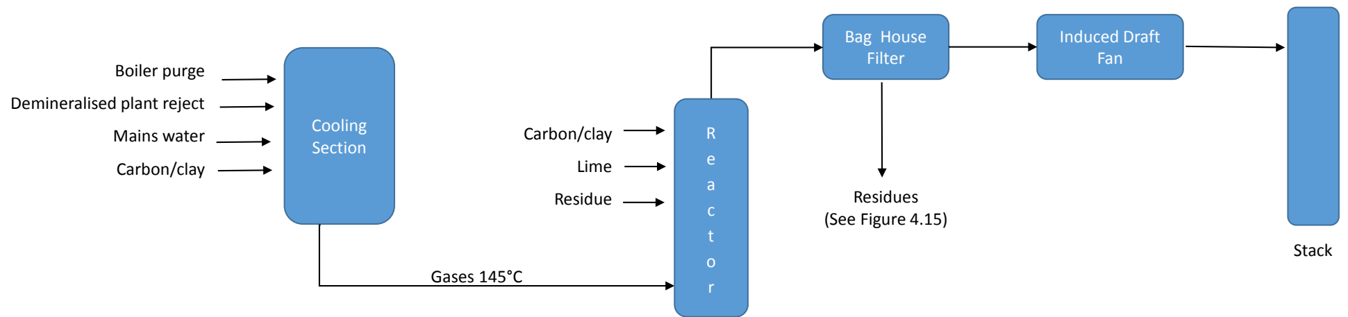
Figure 4.17 Schematic of Cooling Section/Flue Gas Cleaning
