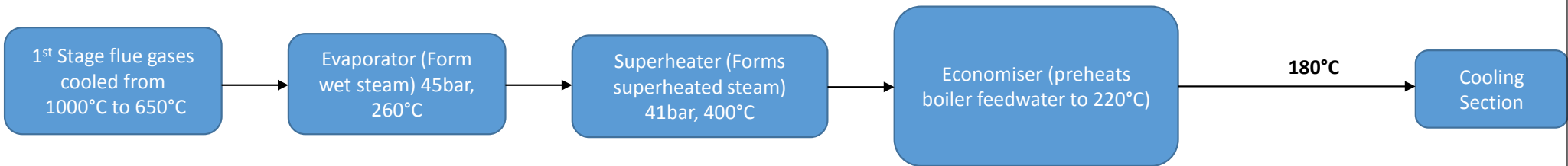
Figure 4.13 Schematic of Boiler
