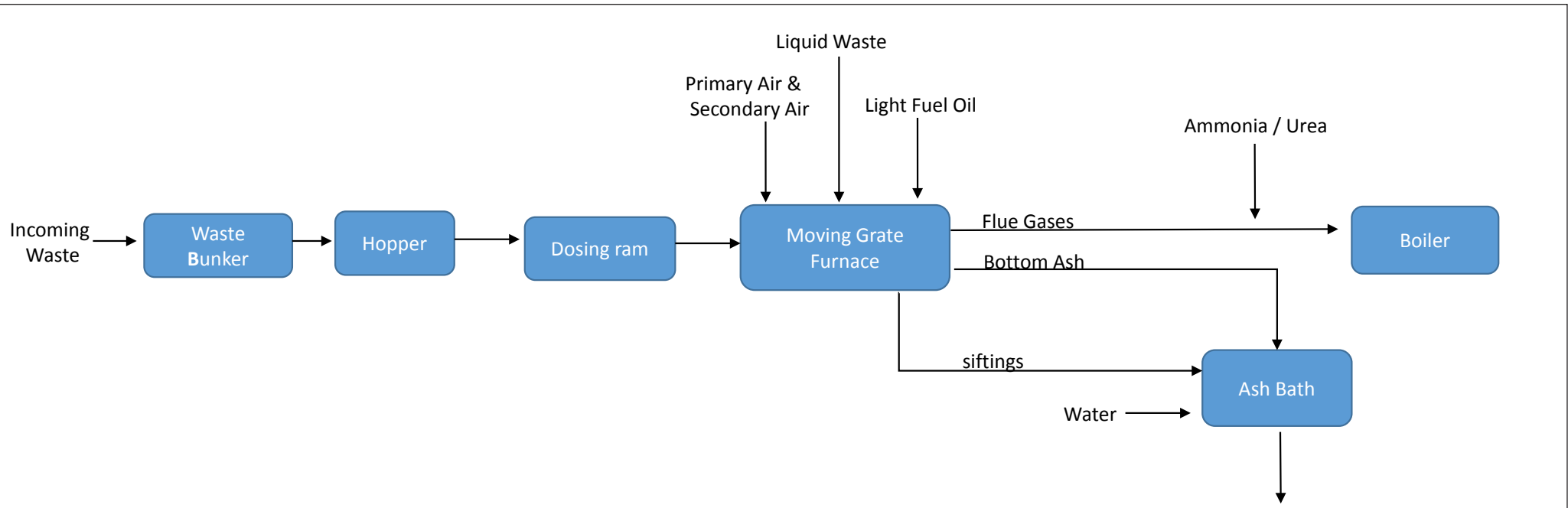
Figure 4.12 Schematic of Moving Grate Furnace
