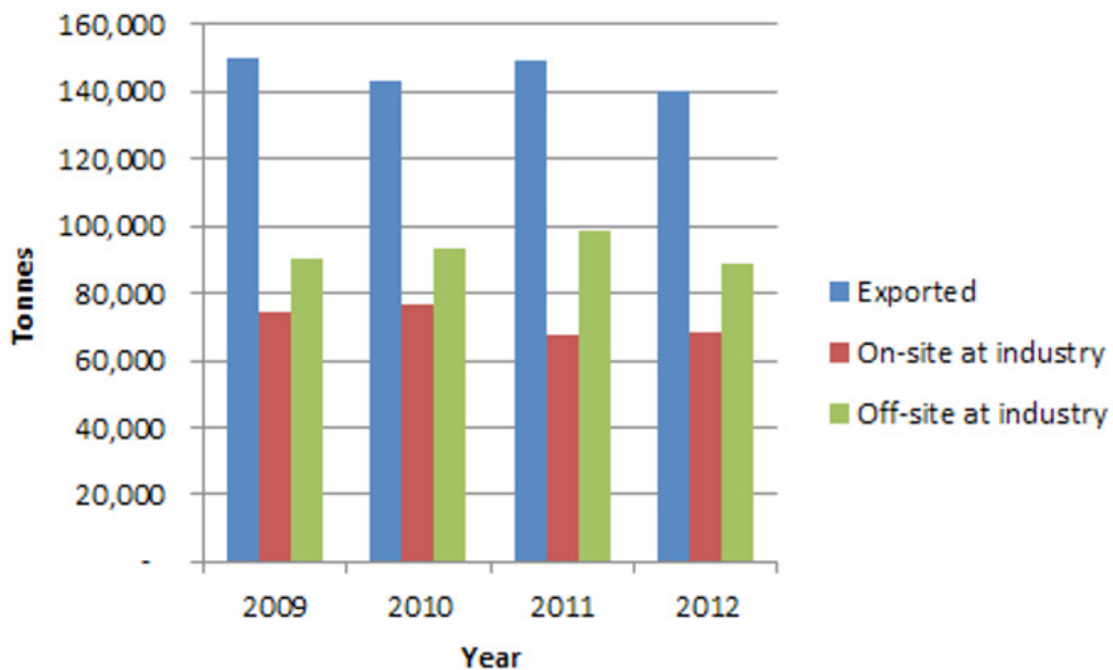
Fig 2.2 - Hazardous Waste Treatment in Ireland 2009-2012
