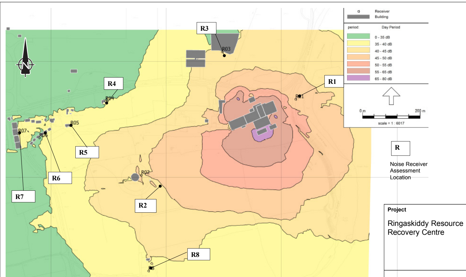
Figure 10.9 Operational Modelled Scenario 1 Calculated Noise Contours
